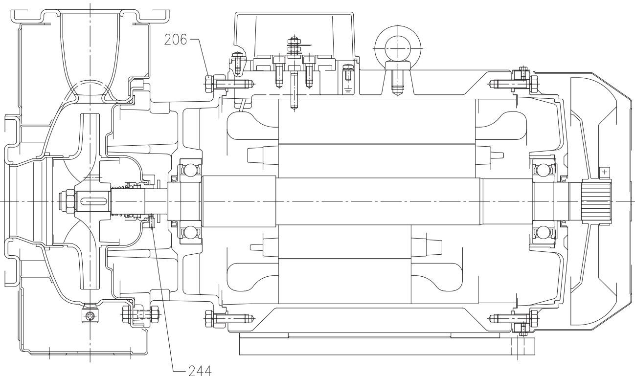
단면도 3(L)M 32, 40, 50, 65 SERIES - from 15 kW and over
