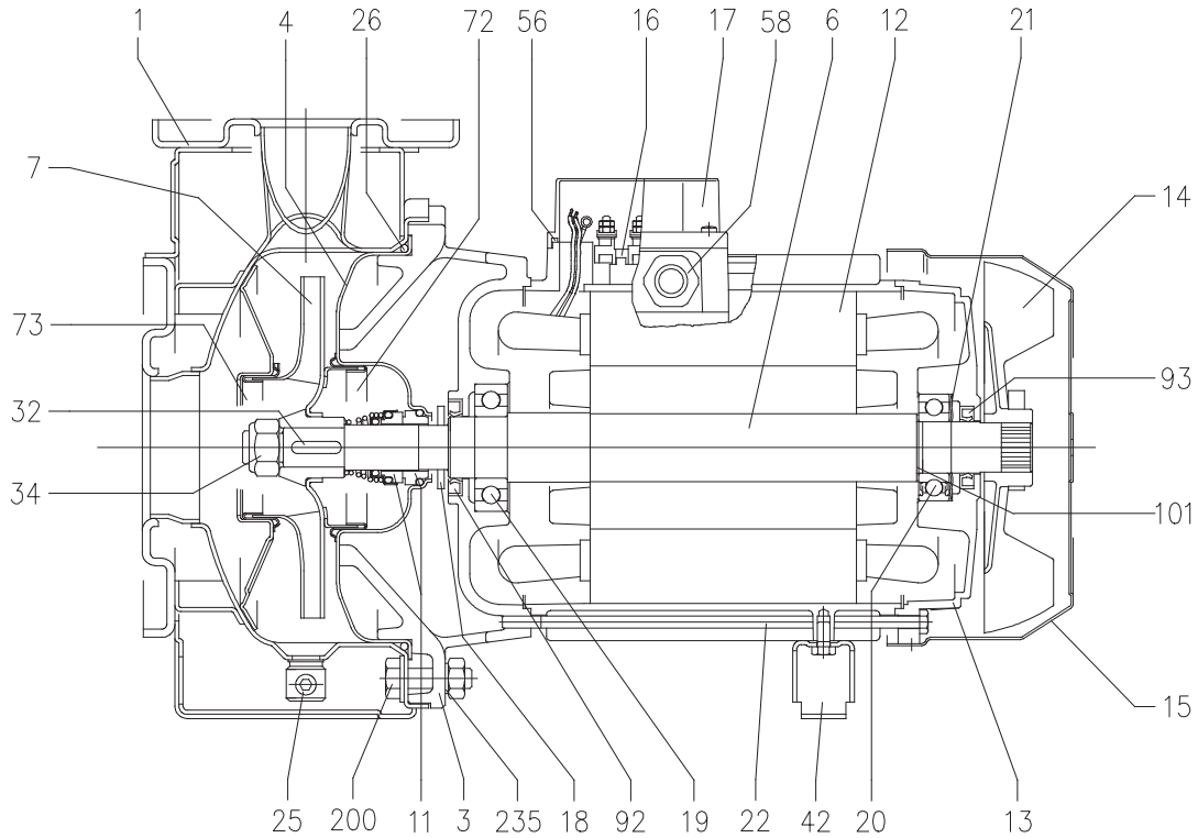
단면도 3(L)M 32, 40, 50, 65 SERIES - from 15 kW and over
